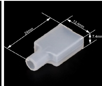
DIMENSIONS OF THE END CAP WITH HOLE / NS-1040-ECH
